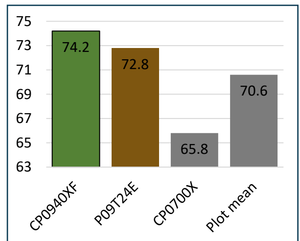
2021 Answer Plot trial. Watertown, SD. SPT-08 set. LSD 3.6.
