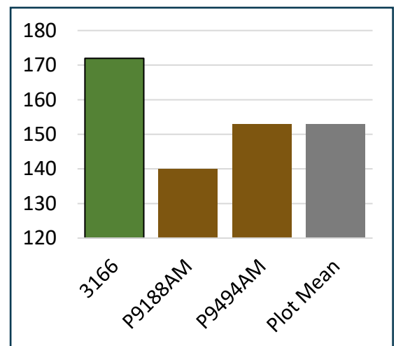
2021 Answer Plot® trial. Ulen, MN. CHT-090 set. LSD 13.3.
