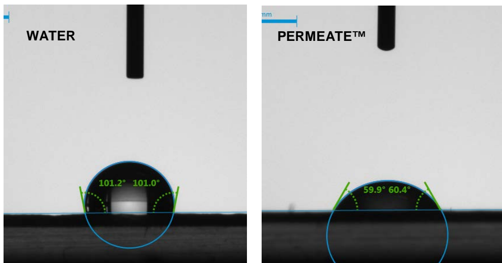
Measured contact angle of water vs. Permeate on wax paper at WinField® United Innovation Center.
